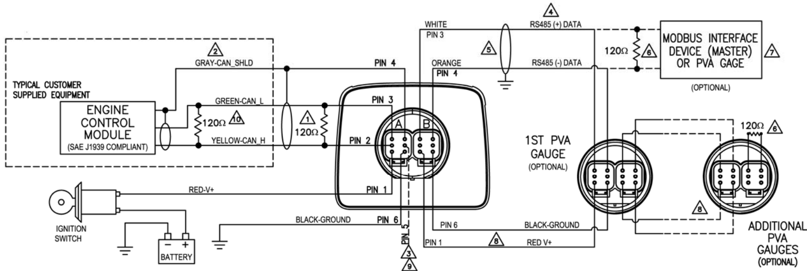
TYPICAL WIRING DIAGRAM
