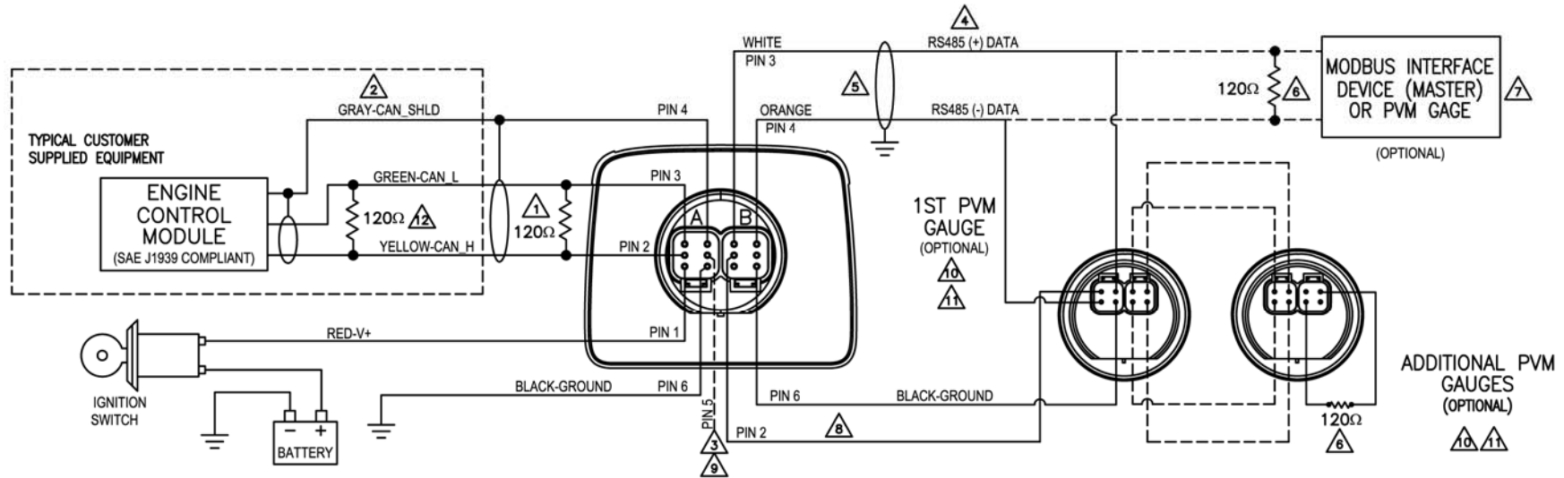
TYPICAL WIRING DIAGRAM
